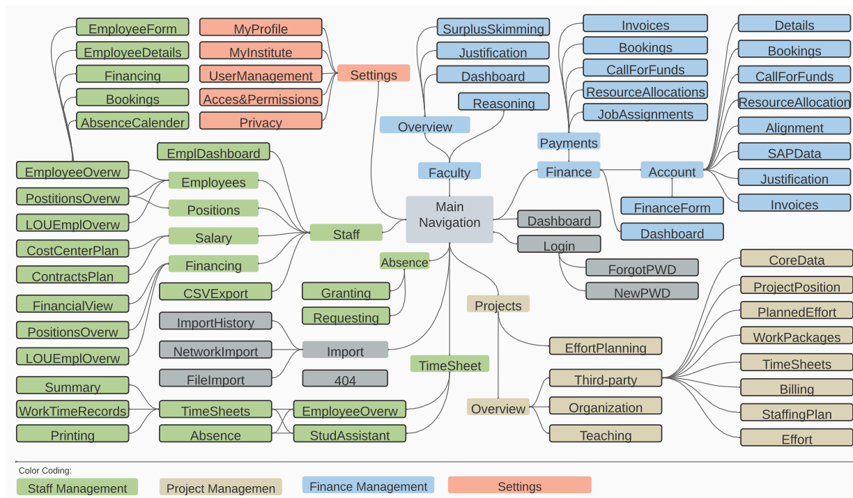
Figure 8: Currently Generated Pages for the Different Segments in MaCoCo.
