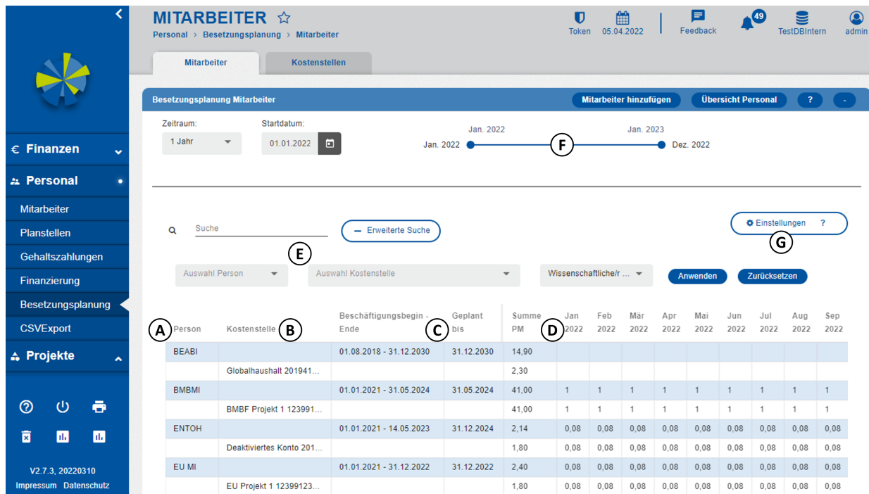
Figure 10: Screenshot of the page for the staff planning (Fig. 8, bottom right)
