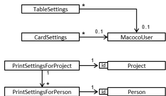
Figure 7: Class Diagram for Settings
