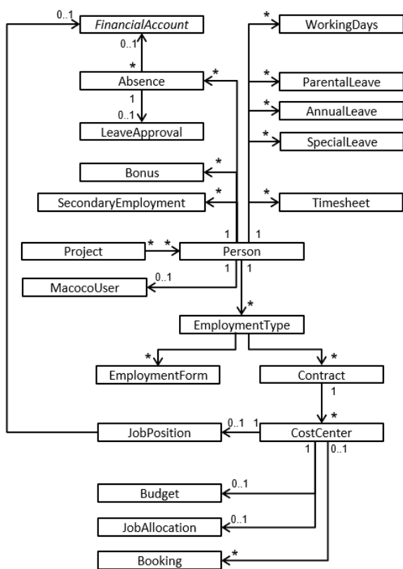
Figure 5: Class Diagram for Staff
