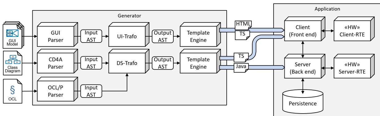
Figure 3: Simplified MontiGem Generator Architecture. Showing the transformation of textual models into abstract representation (AST) that is further transformed and used as input for different Template Engines, that convert the AST into source code.
