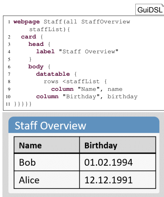
Figure 2: Example GUI model
