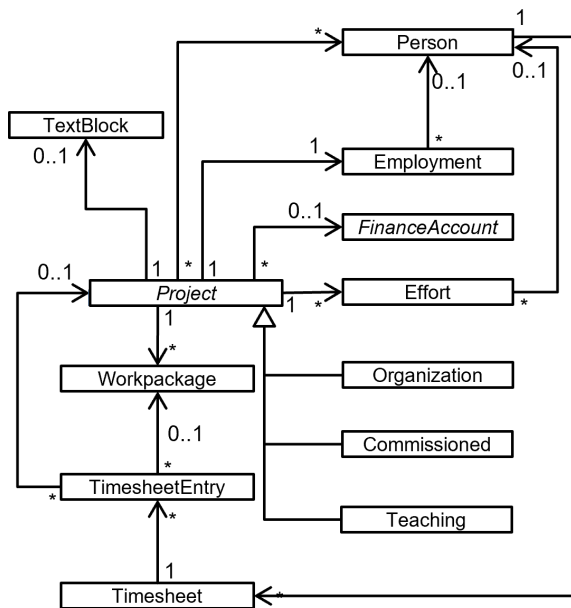
Figure 6: Class Diagram for Project management
