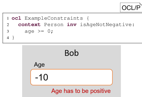
Figure 9: Example OCL/P Model for age validation
